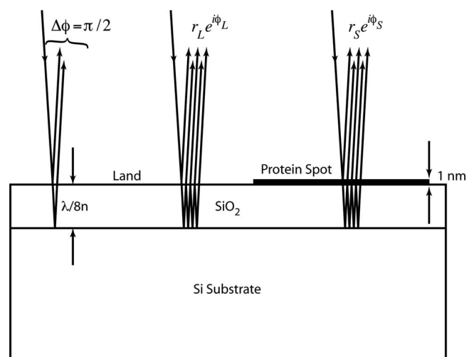
FIG. 9. Thermal oxide on silicon. When the oxide thickness is an eighth-wave, there is a \pi/2 phase difference between the top and bottom reflections (reflection coefficient is purely imaginary). This establishes a quadrature condition that converts the phase load of a thin protein layer directly into intensity at the far-field detector.
