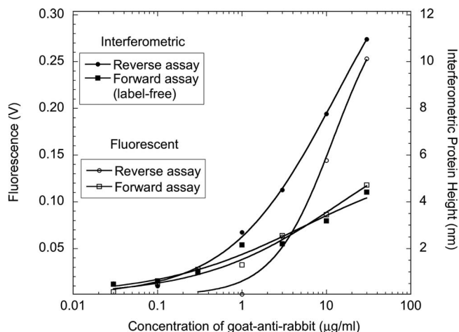
FIG. 20. Comparison of forward and reverse assays using the two channels for interferometry and fluorescence. The interferometry was performed at 488 nm and the fluorescence was at 510 nm. The reverse assay shows a strong amplification for concentrations above 1 \mu\text{g/ml} .
